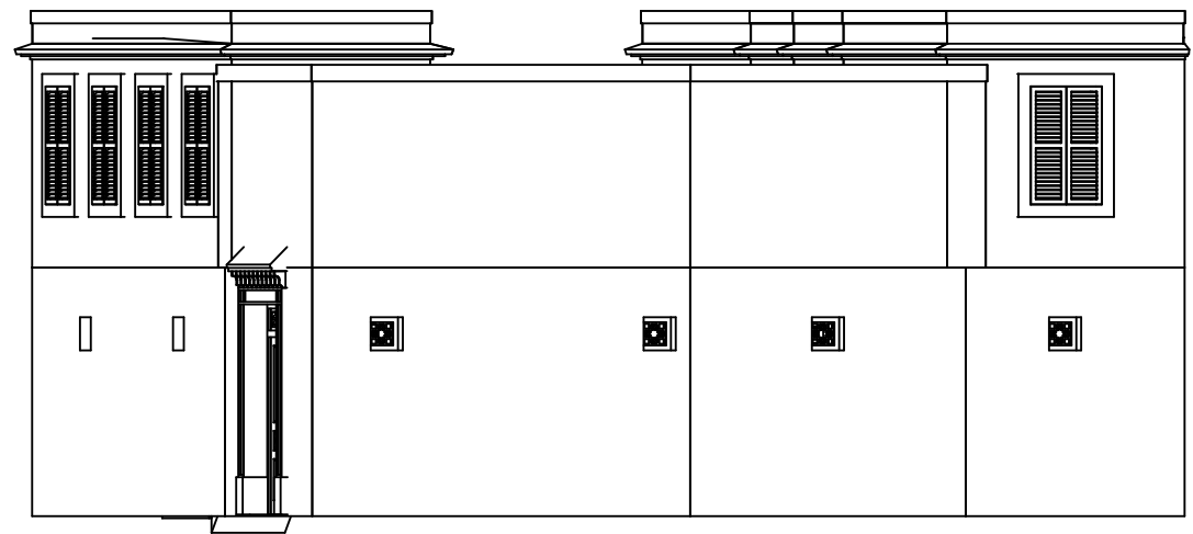
5 Building plot-8 WEST 1:100
