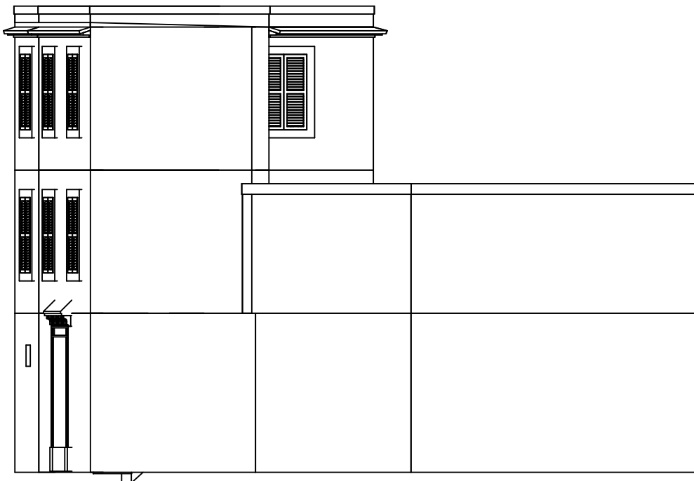
5 Building plot-7 SOUTH 1:100
